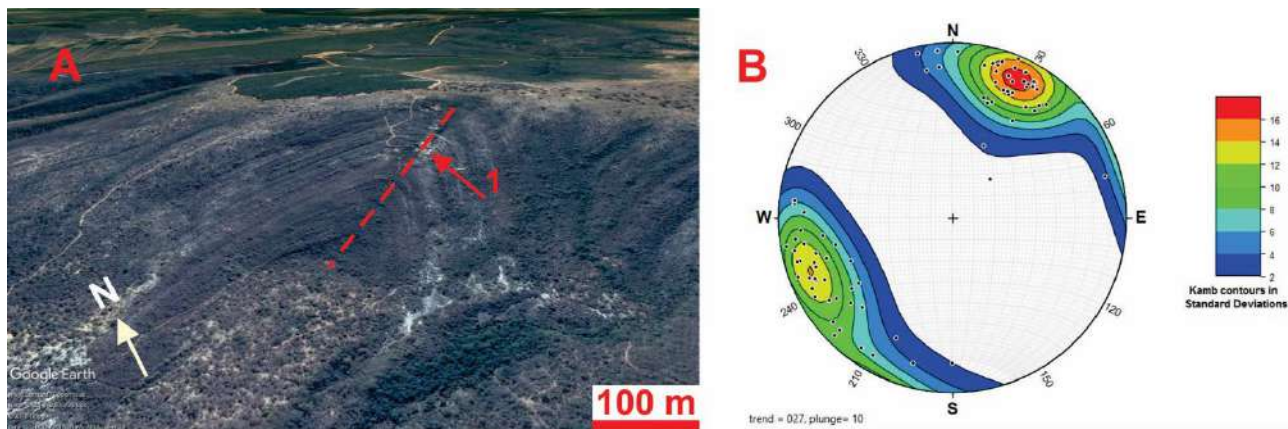
Figure 3. (A) Google Earth view from the tight isoclinal fold present in the quartzites at the Montezuma's amethyst deposit area (red arrow 1), Minas Gerais, where mineralization occurs at the axial surface of the fold (red dashed line). (B) Stereogram of foliation measurements mainly obtained in field by sections perpendicular to the folding axis observed in (A) (n = 70).
