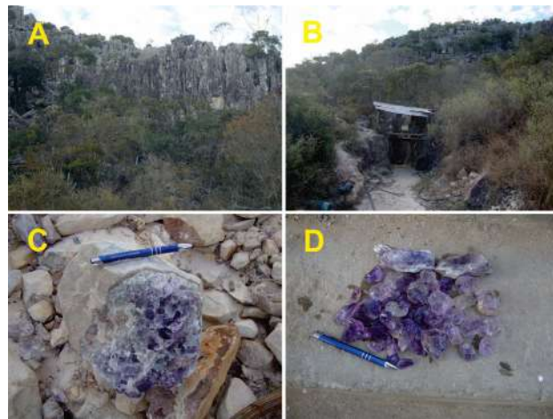
Figure 6. (A) Ruin-shaped quartzites showing a vertical foliation that is typical in Tibério's mine. (B) Aspect of the main pit that goes down to the vein being currently mined at around 30 m deep. (C) Part of an amethyst vein in the host quartzite. (D) Hand-selected amethyst parcel with deeper color.
