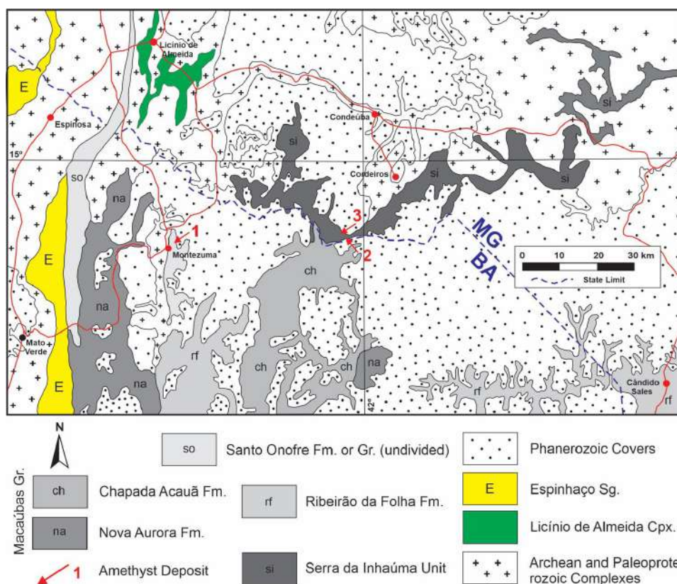
Figure 1. Geology of the neighboring region between the MG and BA states with several recognized units of the Macaúbas Group (Neoproterozoic) highlighted in shades of gray, and the “Serra de Inhaúma” (Paleoproterozoic?) and “Santo Onofre” (Neoproterozoic) sequences within this context (according to Souza et al., 2009a, 2009b, respectively Brasília and Salvador sheets, partial and modified). Amethyst deposits: 1, Montezuma (MG); 2, Coruja (BA); and 3, Tibério (BA).
