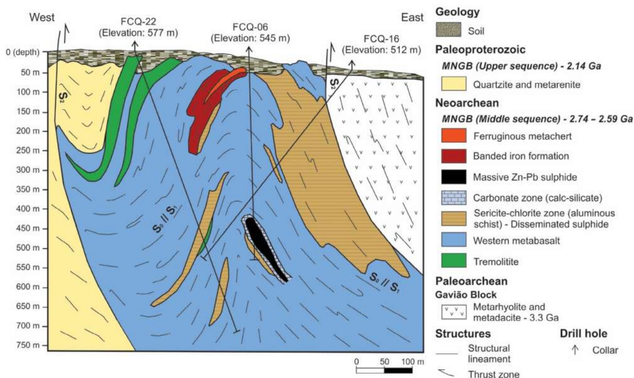
Figure 7. Geological cross section of the Fazenda Coqueiro volcanic-hosted massive sulfide deposit showing the antiform, the distribution of the western metabasalt, and the carbonate and sericite-chlorite zones based on outcrops and drill core descriptions. The site of the geological cross section is represented in the geological map of Figure 3.
