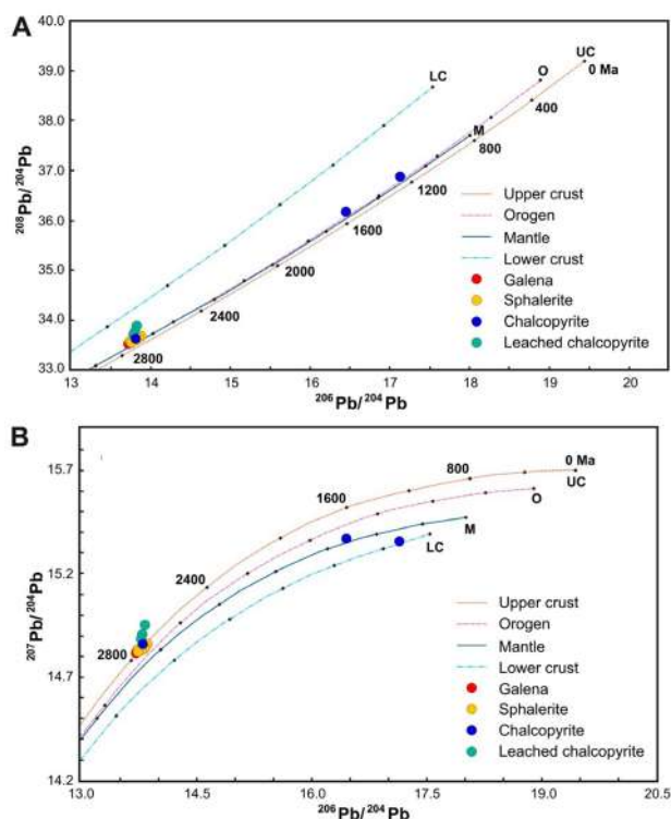
Figure 12. (A) Thorogenic and (B) uranogenic diagrams (Zartman and Doe, 1981) used for source study of the sphalerite, galena and chalcopyrite samples from the Fazenda Coqueiro volcanic-hosted massive sulfide deposit.
