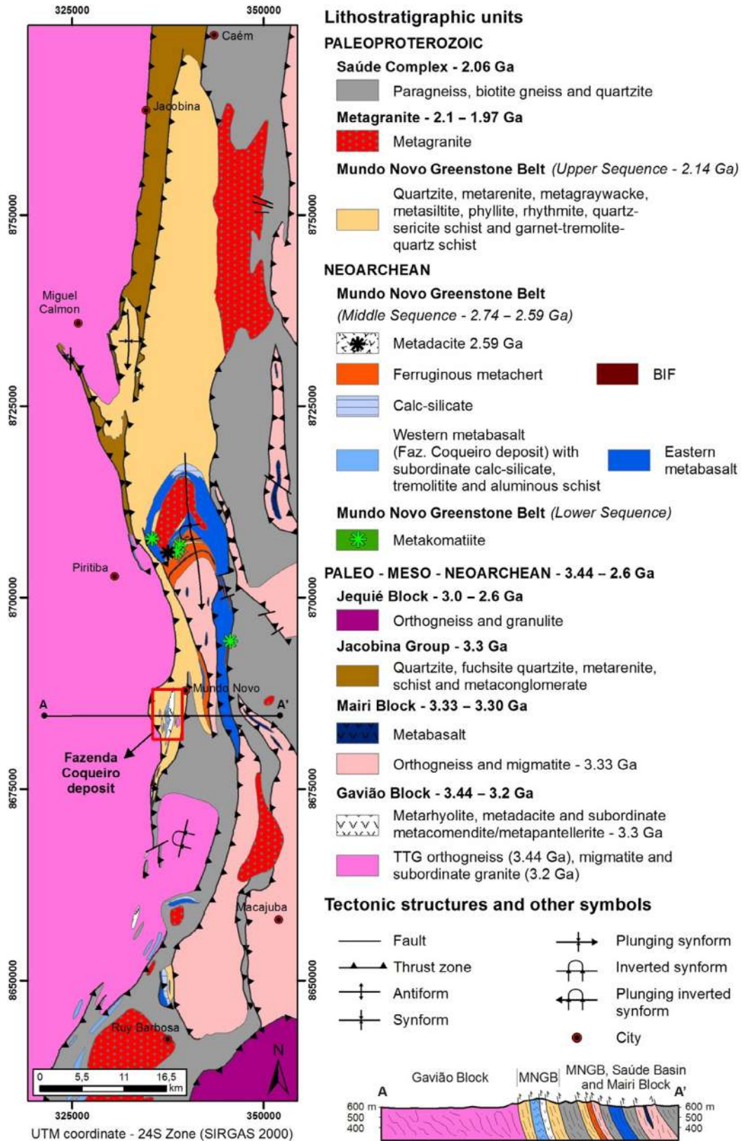
Figure 2. Geological map of the Mundo Novo greenstone belt and adjoining units. From Spreatico et al. (2019) and updated with data from the present work.
