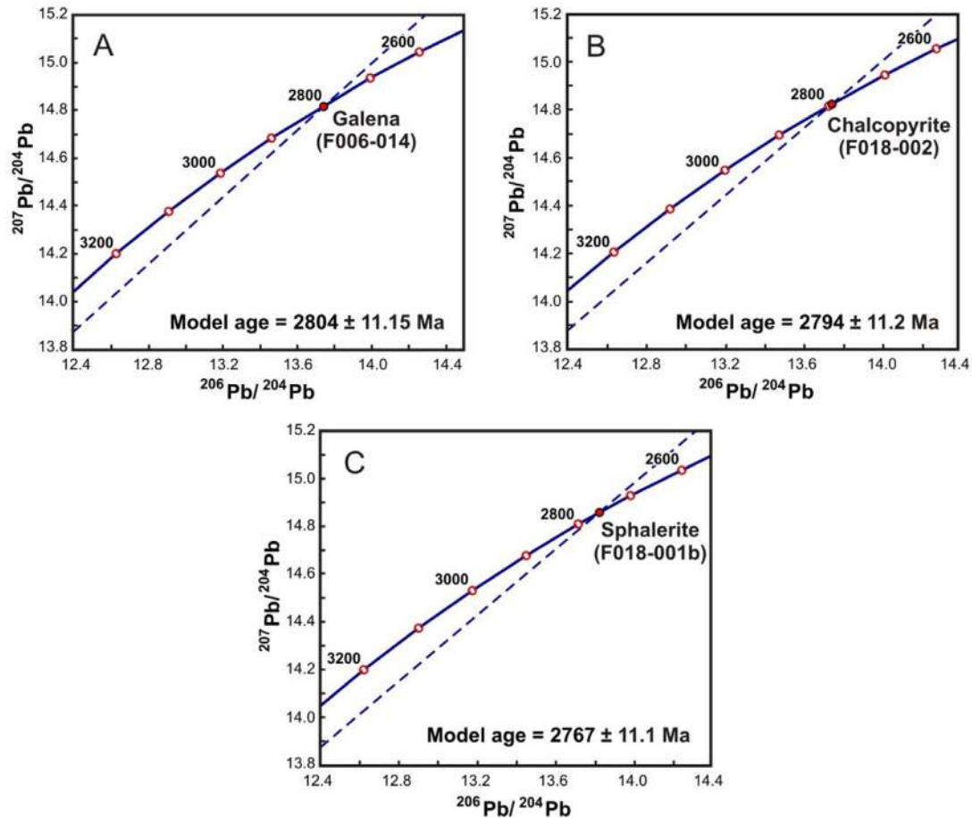
Figure 10. ^{206}\text{Pb}/^{204}\text{Pb} vs. ^{207}\text{Pb}/^{204}\text{Pb} diagram for model age determination for three sulfide samples from the Fazenda Coqueiro volcanic-hosted massive sulfide deposit: (A) Galena sample from the silica-rich level in the sericite-chlorite zone. (B) Chalcopyrite sample from the carbonate and massive sulfide zone. (C) Sphalerite sample from the carbonate and massive sulfide zone.
