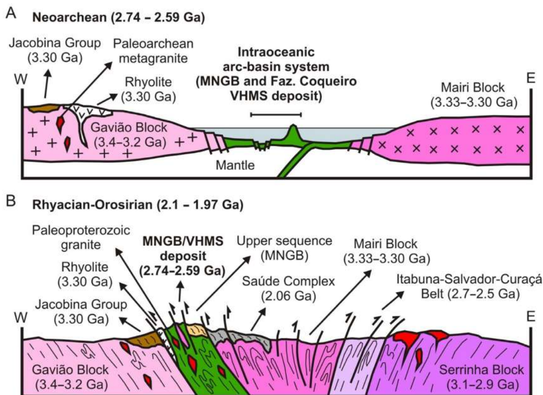
Figure 14. Regional geological setting of the Mundo Novo greenstone belt (MNGB) and Fazenda Coqueiro volcanic-hosted massive sulfide deposit. (A) Deposit formation in an intraoceanic arc-basin system at 2,747 Ma. (B) Final result of the Rhyacian-Orosirian tectonic event that compressed the MNGB and the Fazenda Coqueiro deposit between cratonic blocks in the eastern São Francisco Craton.
