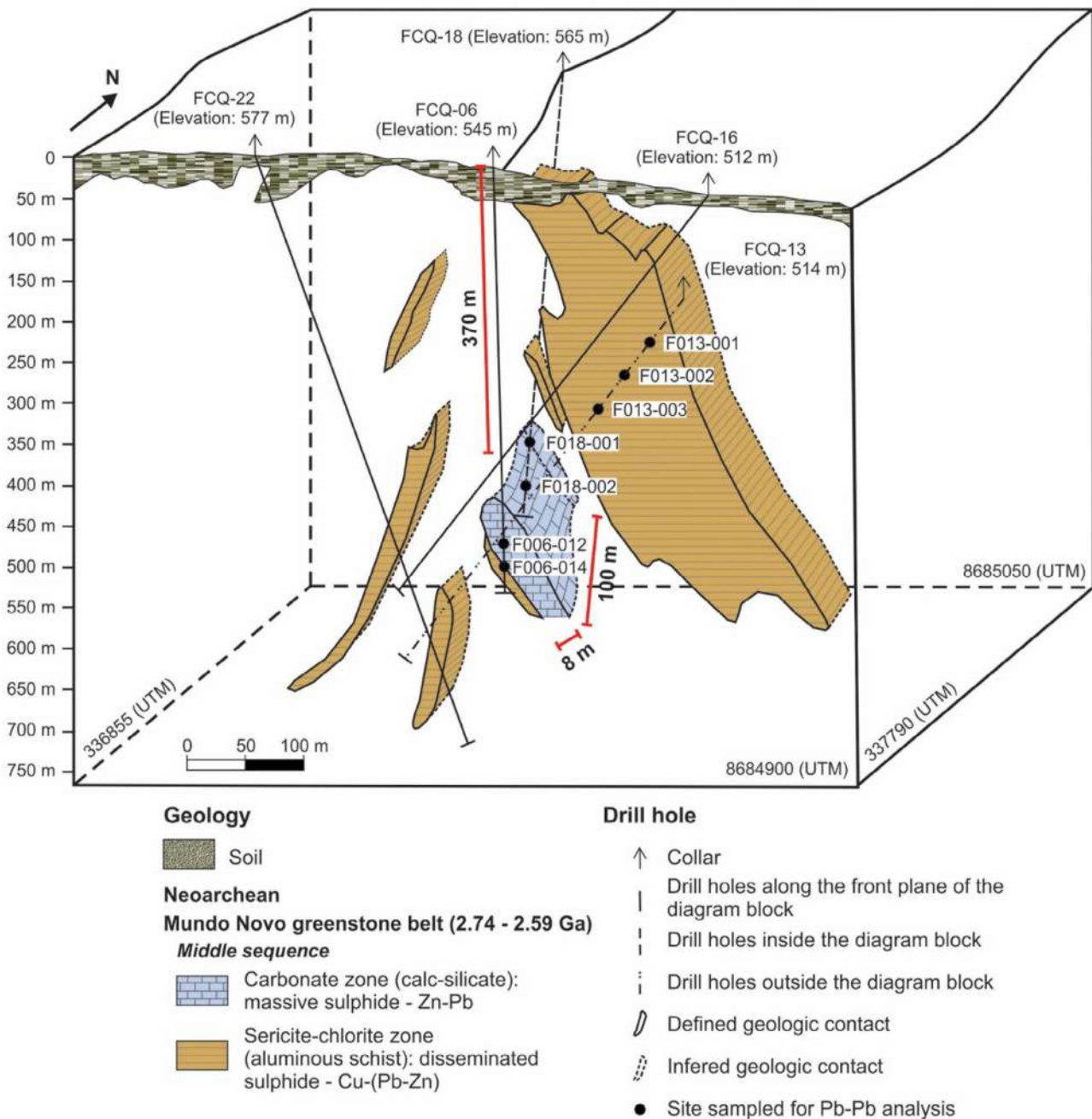
Figure 8. Block diagram of the Fazenda Coqueiro volcanic-hosted massive sulfide deposit showing the distribution and geometry interpreted for metamorphosed hydrothermal alteration zones, the associated mineralization and the sites sampled for Pb-Pb analysis. See Appendix 1 for collar coordinates.
