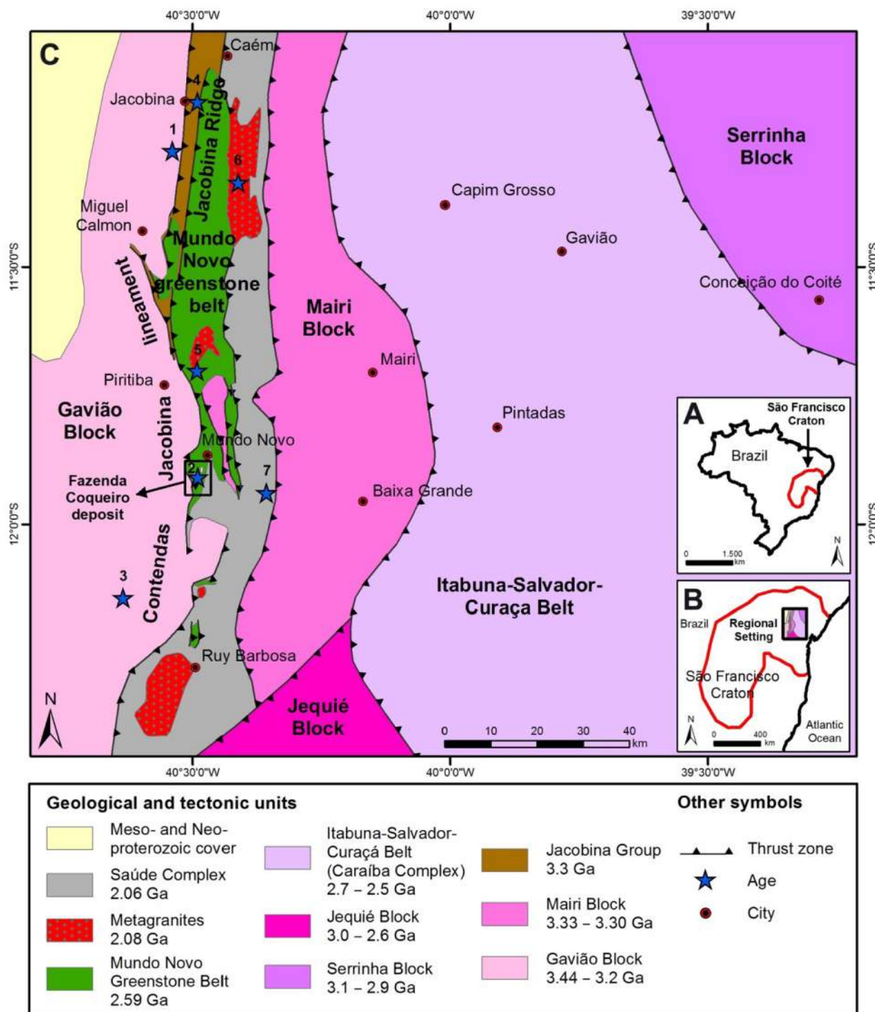
Figure 1. (A) Location of the São Francisco Craton in NE Brazil. (B) Regional setting in the eastern portion of the São Francisco Craton. (C) Regional tectonic setting where the Mundo Novo greenstone belt (MNGB) and the Fazenda Coqueiro deposit are inserted (modified from Barbosa and Sabaté, 2002, 2003, 2004). Ages at the points highlighted on the map: (1) 3,442 \pm 2 Ma (U-Pb zircon, TTG; Mougeot, 1996); (2) 3,303 \pm 11 Ma (U-Pb zircon, metarhyolite from the Gavião Block obtained by Zincone et al., 2016); (3) 3,292 \pm 3 Ma (U-Pb zircon, metagranite from the Gavião Block obtained by Zincone et al., 2016); (4) 3,500–3,220 Ma (U-Pb zircon, quartzite from the Jacobina Group obtained by Teles et al., 2015); (5) 2,595 \pm 21 Ma (U-Pb zircon, metadacite from the MNGB obtained by Spreafico et al., 2019); (6) 2,080 \pm 18 Ma (U-Pb monazite, Cachoeira Grande granite obtained by Leite, 2002); (7) 2,068 \pm 12 Ma (U-Pb zircon, biotite schist from the Saúde Complex obtained by Zincone et al., 2017).
