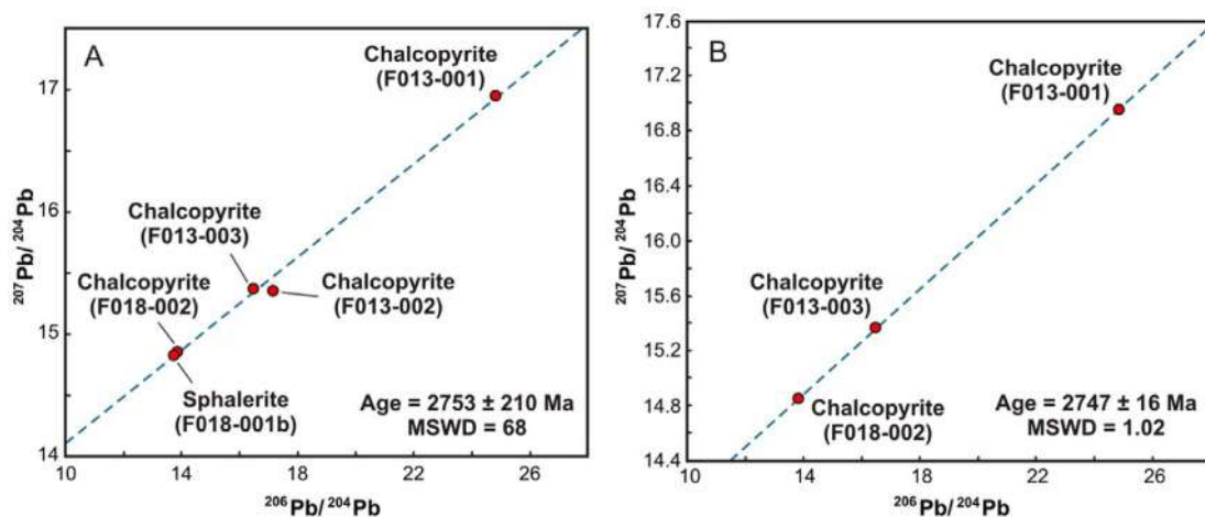
Figure 11. Detail of the isochron on the ^{206}\text{Pb}/^{204}\text{Pb} vs. ^{207}\text{Pb}/^{204}\text{Pb} diagram to determine the crystallization age of sulfides from the Fazenda Coqueiro volcanic-hosted massive sulfide deposit (MSWD). (A) Detailed isochron using five sulfide samples yields an age of 2,753 \pm 210 Ma with, however, a high MSWD of 68. (B) Detailed isochron using one sample of chalcopyrite from the massive sulfide zone (F018-002) and two samples of chalcopyrite from the disseminated sulfide zone in the sericite-chlorite zone (F013-001 and F013-003) that yields an age of 2,747 \pm 16 Ma and MSWD of 1.02.
