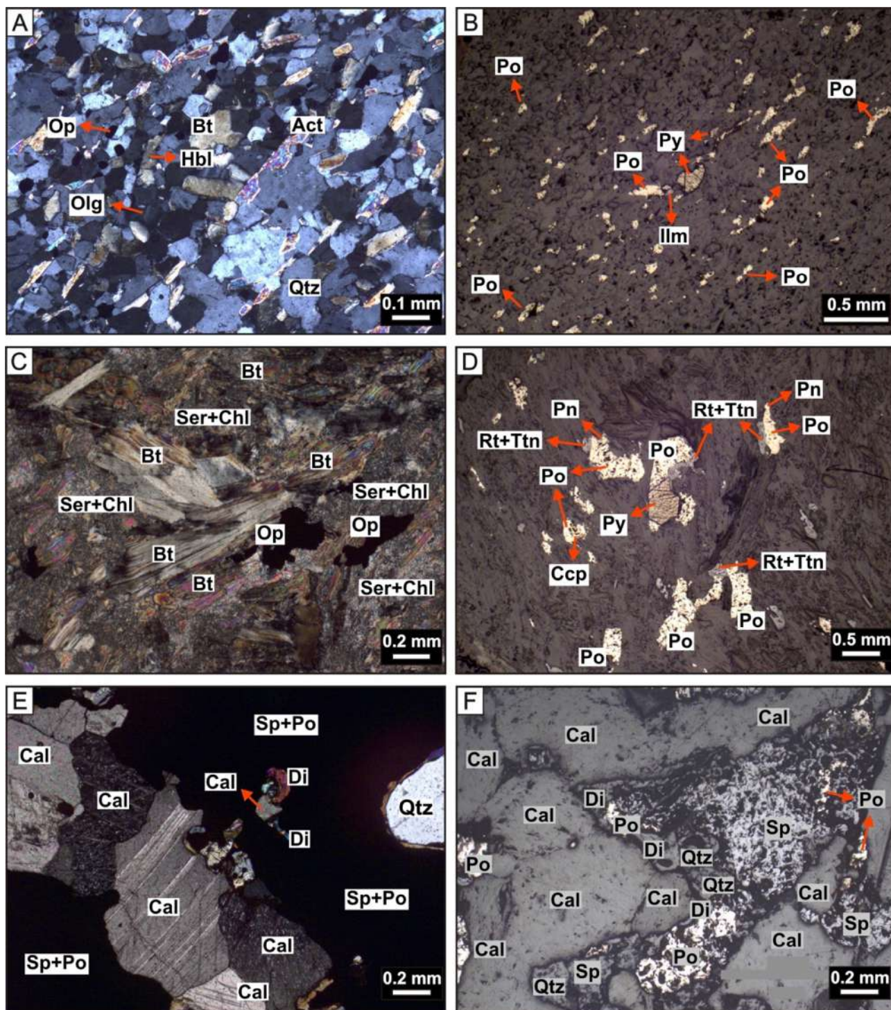
Figure 5. Petrographic images of the western metabasalt and metamorphosed hydrothermal alteration zones. (A) Very fine-grained and polygonal granonematoblastic microstructure and oriented grains in the western metabasalt (cross polarized light). (B) Traces of elongated and oriented pyrrhotite and pyrite grains in the western metabasalt (reflected light). (C) Sericite-chlorite zone composed of biotite, chlorite, sericite, and opaque minerals (plane polarized light). (D) Elongated and oriented sulfide grains in the sericite-chlorite zone (reflected light). (E) Intergrowth of silicates, carbonate and sulfides in the carbonate zone (cross polarized light). (F) Intergrowth of sphalerite, pyrrhotite, calcite, quartz, and diopside in the carbonate zone (reflected light).
