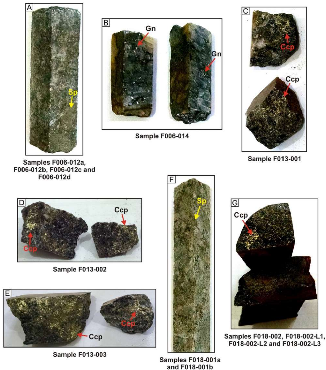
Figure 9. Drill cores used for Pb-Pb geochronological study of sulfides from the Fazenda Coqueiro volcanic-hosted massive sulfide deposit. (A) Carbonate zone with massive sphalerite from which four samples were obtained for the source study. (B) Silica-rich core level in the sericite-chlorite zone with galena sampled for model age study. (C, D, and E) Sericite-chlorite zone with disseminated chalcopyrite sampled for crystallization age and source study. (F) Carbonate-rich core with massive sphalerite from which two samples were obtained for model and crystallization ages and source study. (G) Carbonate zone core with chalcopyrite from which four samples (whole digestion and leached fractions) were obtained for model and crystallization ages and source study.
