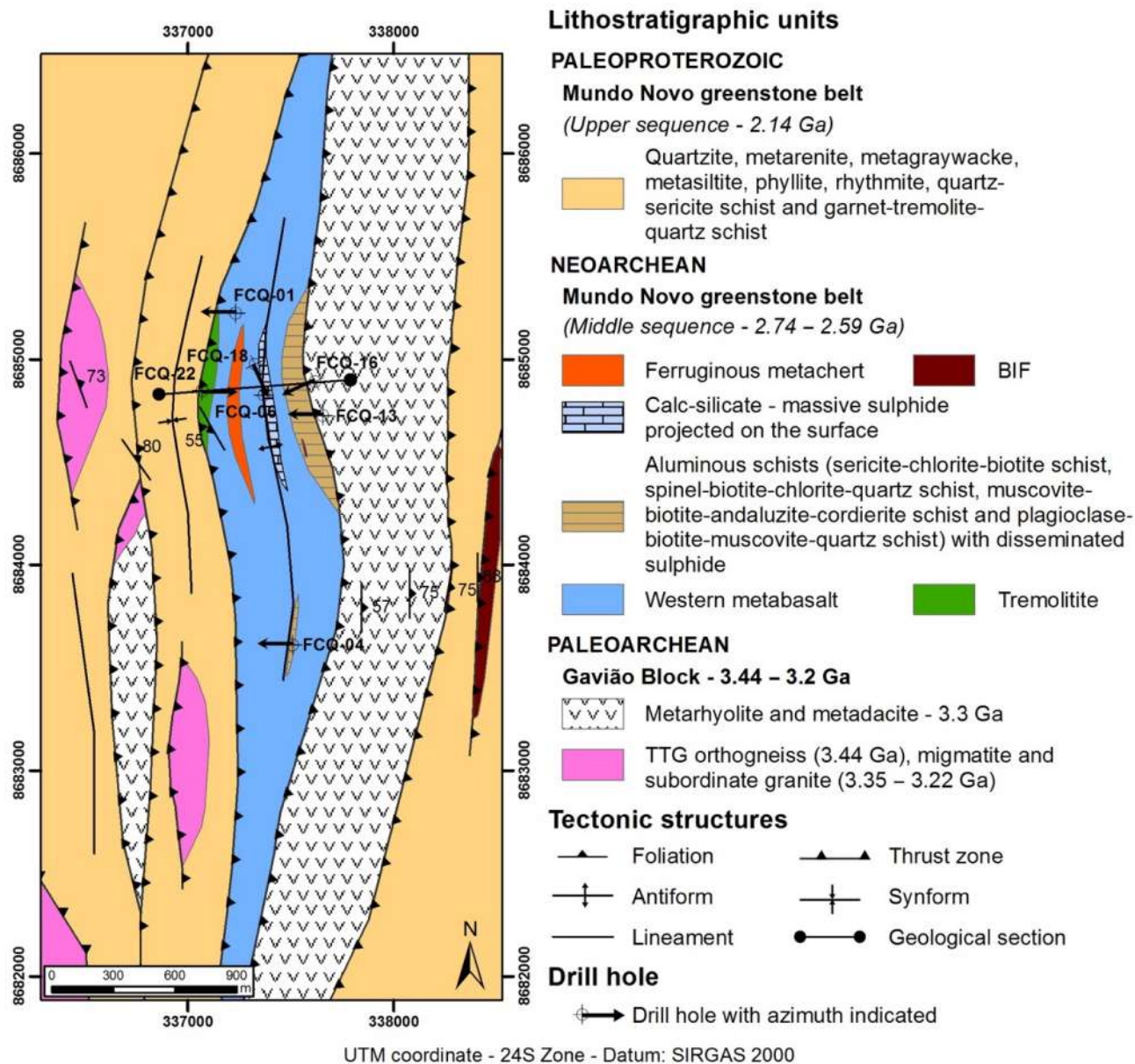
Figure 3. Geological map of the Fazenda Coqueiro volcanic-hosted massive sulfide deposit and the drill hole sites where the sulfide samples were collected for Pb-Pb analyses.
