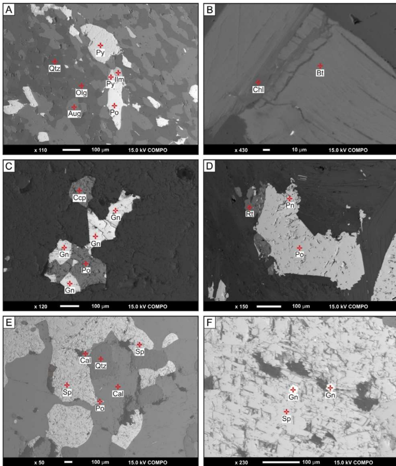
Figure 6. Backscattered electron images with the analytical spots in the core samples of the Fazenda Coqueiro volcanic-hosted massive sulfide deposit. (A) Intergrowth of pyrite and pyrrhotite, and very fine-grained and polygonal granonematoblastic microstructure in the western metabasalt. (B) Replacement of chlorite by biotite in the sericite-chlorite zone. (C) Intergrowth of chalcopyrite, galena and pyrrhotite in the silica-rich level in the sericite-chlorite zone. (D) Intergrowth of pyrrhotite, pentlandite and rutile in the sericite-chlorite zone. (E) Intergrowth of sphalerite, pyrrhotite, calcite, and quartz in the carbonate zone. (F) Inclusions of galena in sphalerite grains hosted in the carbonate zone.
