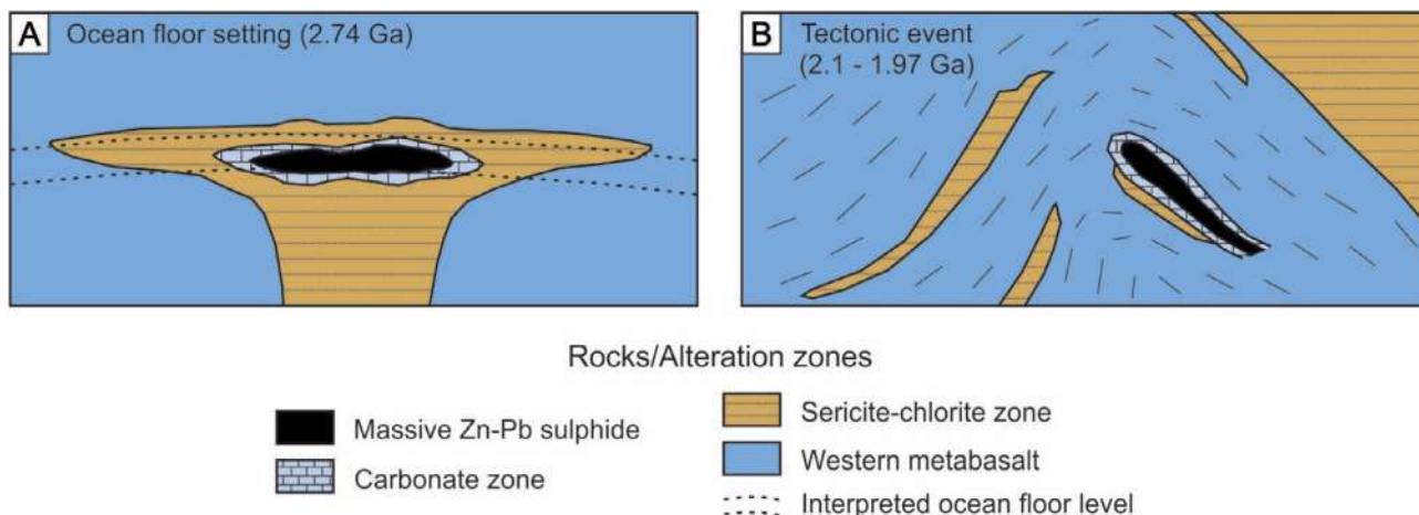
Figure 13. Metallogenic model of the Fazenda Coqueiro volcanic-hosted massive sulfide deposit. (A) Interpreted distribution and relation among the volcanic rock, massive sulfide and hydrothermal alteration zones in the ocean floor setting at 2,747 Ma. (B) Positioning of the massive sulfide lens and alteration zones after the Rhyacian-Orosirian tectonic event.
